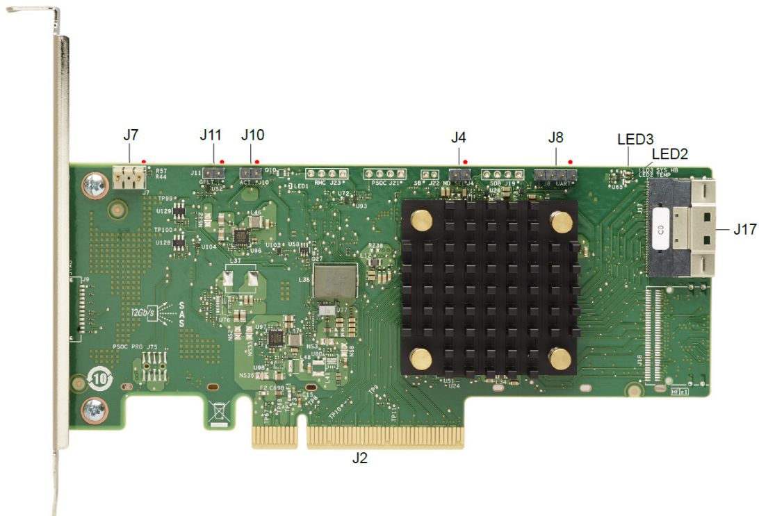
Figure 1: Card Layout for the ThinkSystem RAID 545-8i PCIe Gen4 12Gb Adapter
